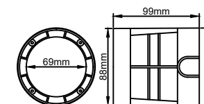
Back Box
